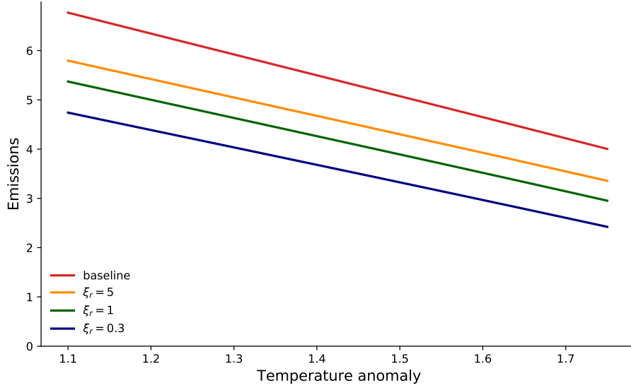
Figure 9: Emissions as a function of the temperature anomaly for different penalty configurations. The thresholds are \underline{y} = 1.75 and \bar{y} = 2.25 . We limit the domain of the function to be 1.1 - 1.75 because for larger temperature anomalies the Poisson event may be realized.
